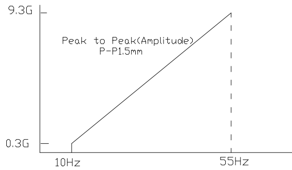
FIG3 VIBRATION TEST
