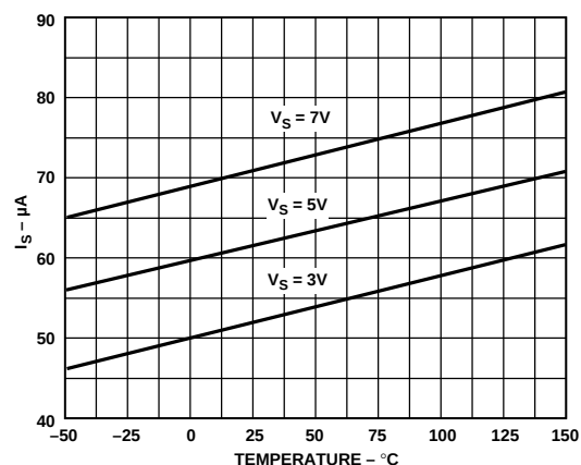
Figure 5. Supply Current vs. Temperature ( V_{OUT} = \text{HIGH} )
